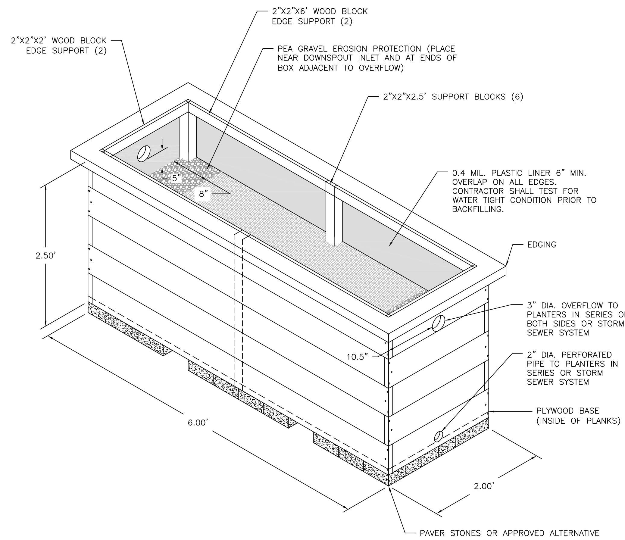
4.1 DOWNSPOUT PLANTER ISOMETRIC DT-4 N.T.S.
