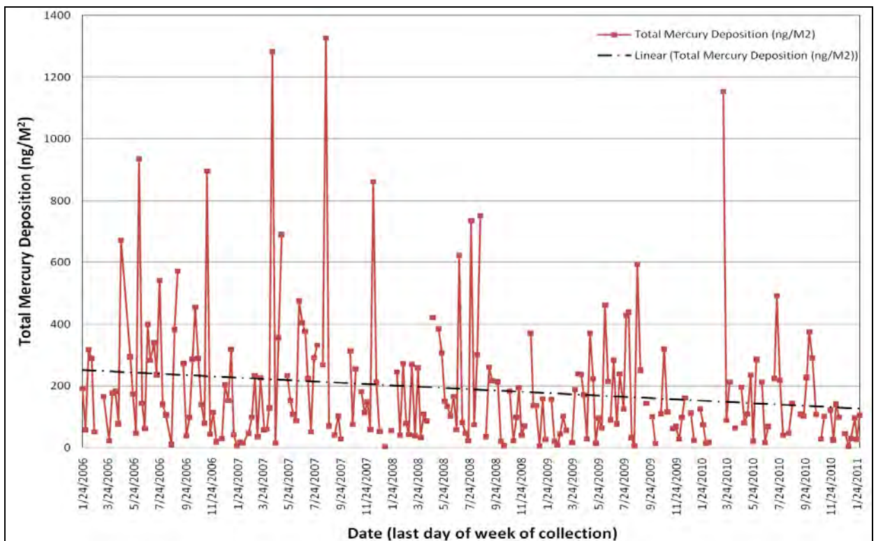
Figure 2d: Total Mercury Deposition in Wet Deposition at New Brunswick
