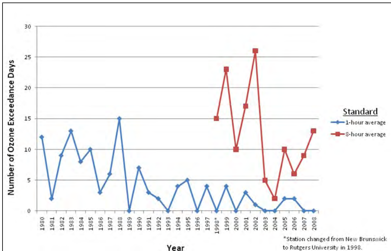
Figure 2b: Ozone Exceedance Days
