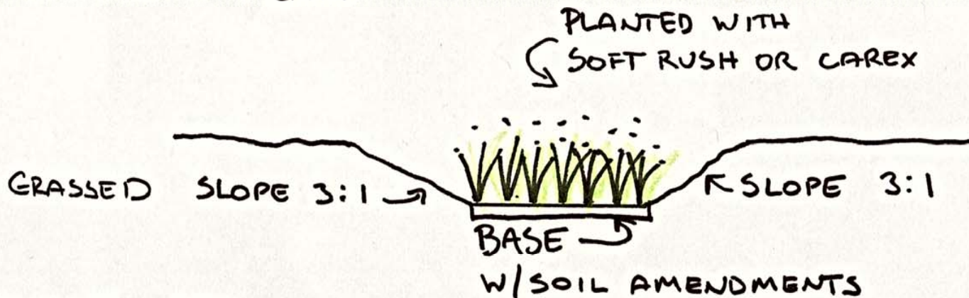
BIOSWALE - CROSS SECTION
