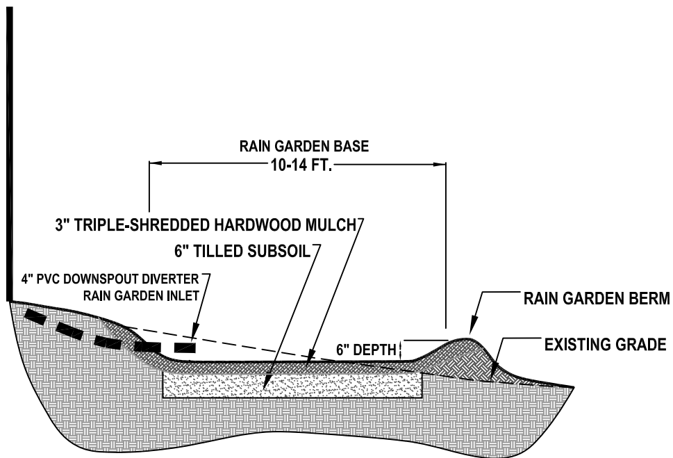
RAIN GARDEN CROSS SECTION
