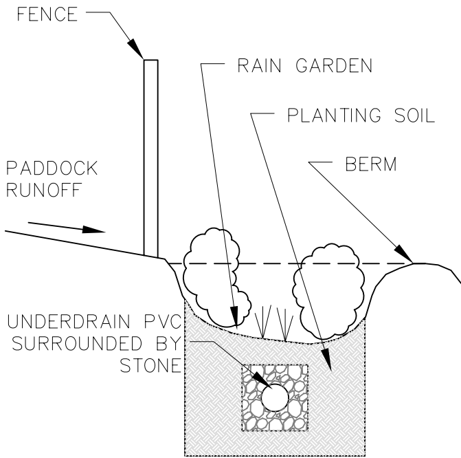
COMPLETED RAIN GARDEN
