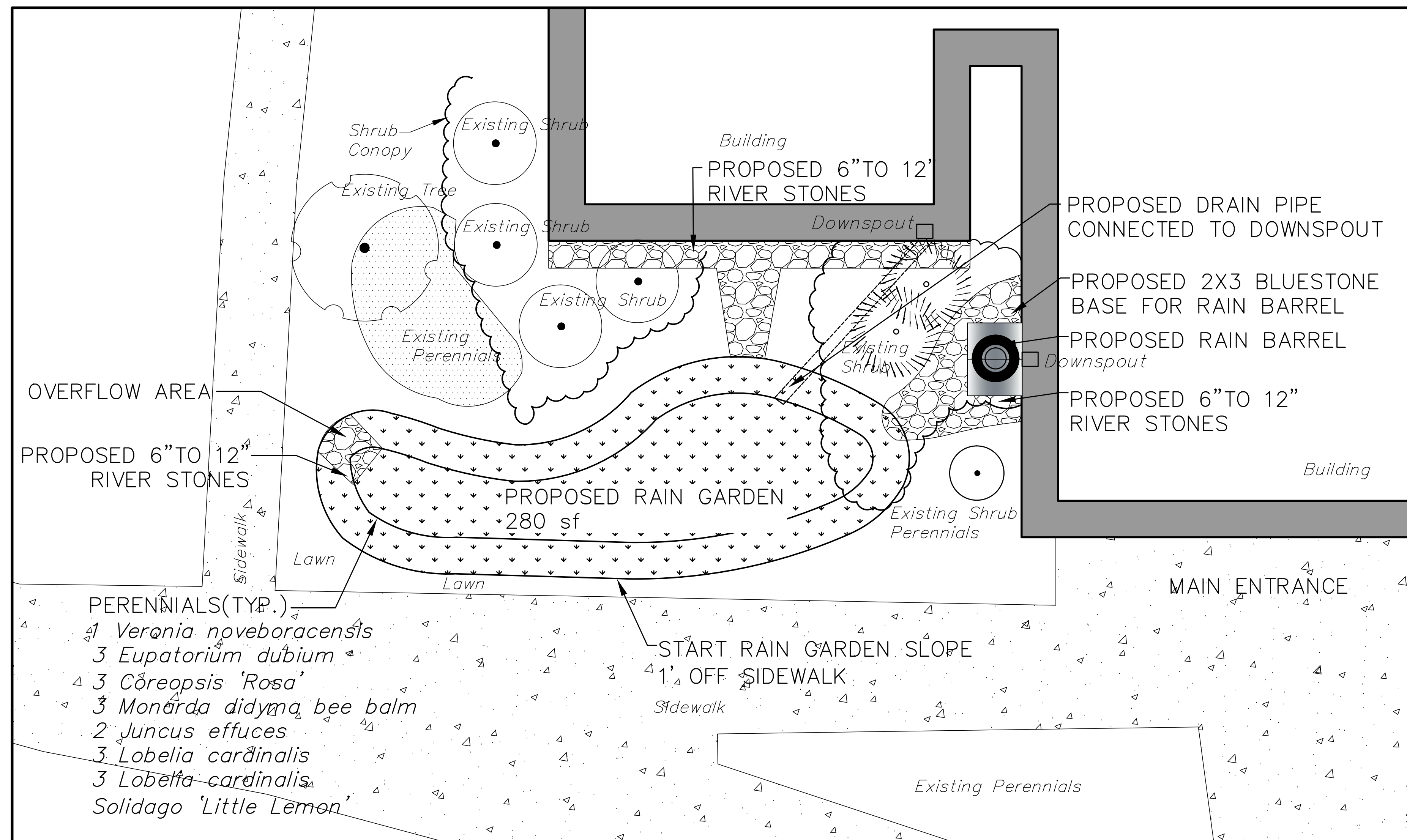
PLAN
