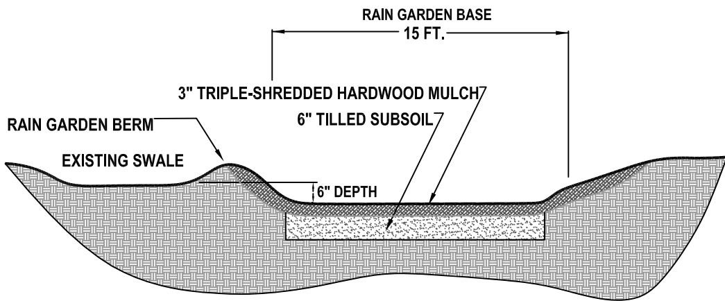
RAIN GARDEN CROSS SECTION
